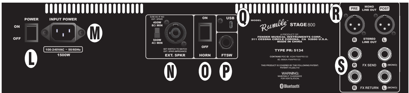
Rumble Stage 800 rear panel shown; Rumble Studio 40 rear panel has same features except for external speaker output and impedance switch (N).
